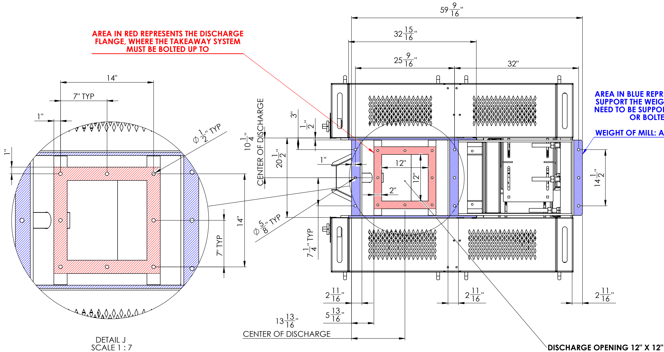
BOTTOM VIEW
