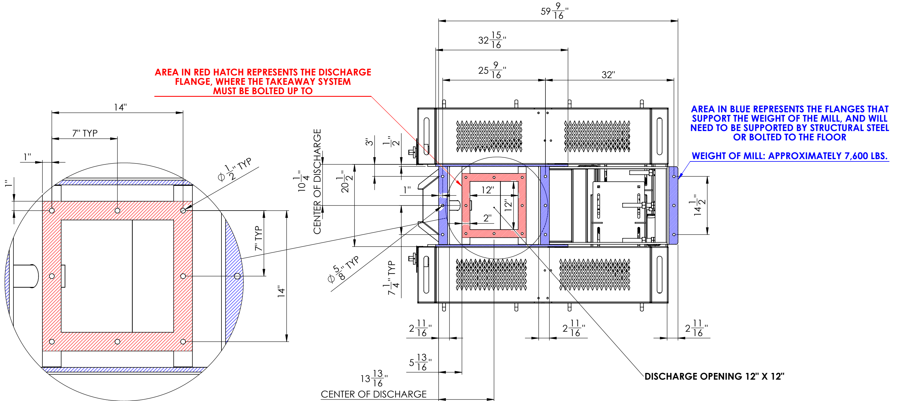
DETAIL I SCALE 1 : 6
